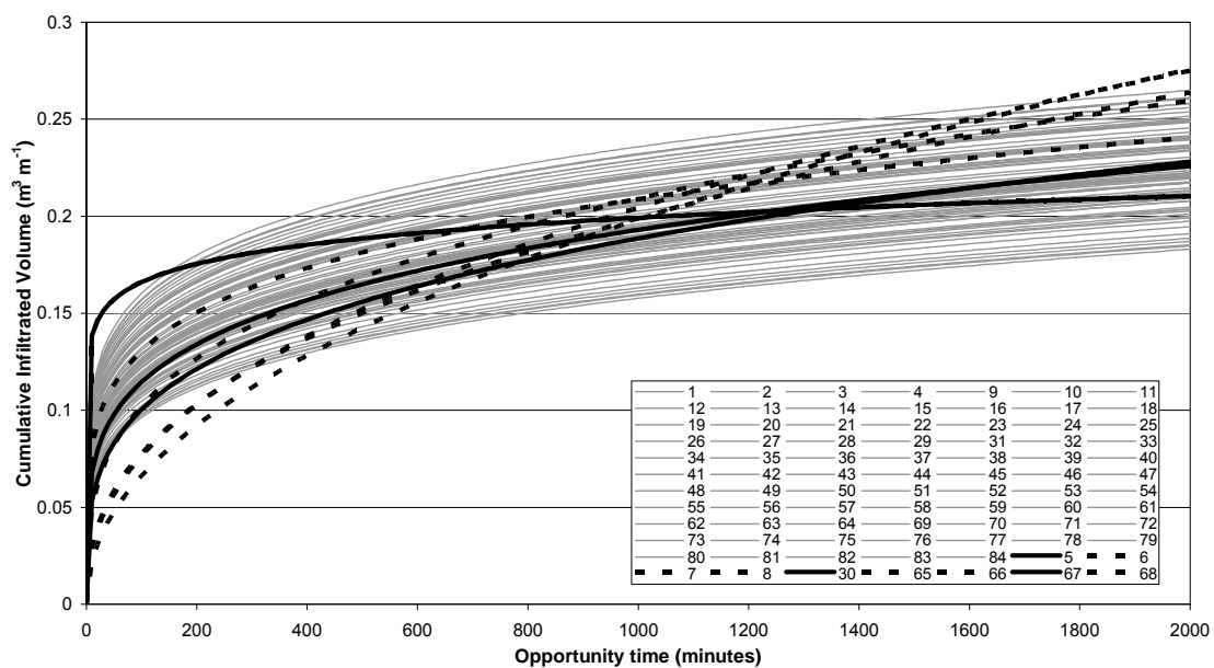
Figure 3 – Infiltration curves from IPARM (Black) and predictive technique (grey)
