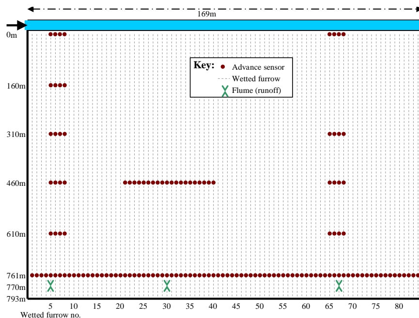
Figure 1 - Field trial site layout
